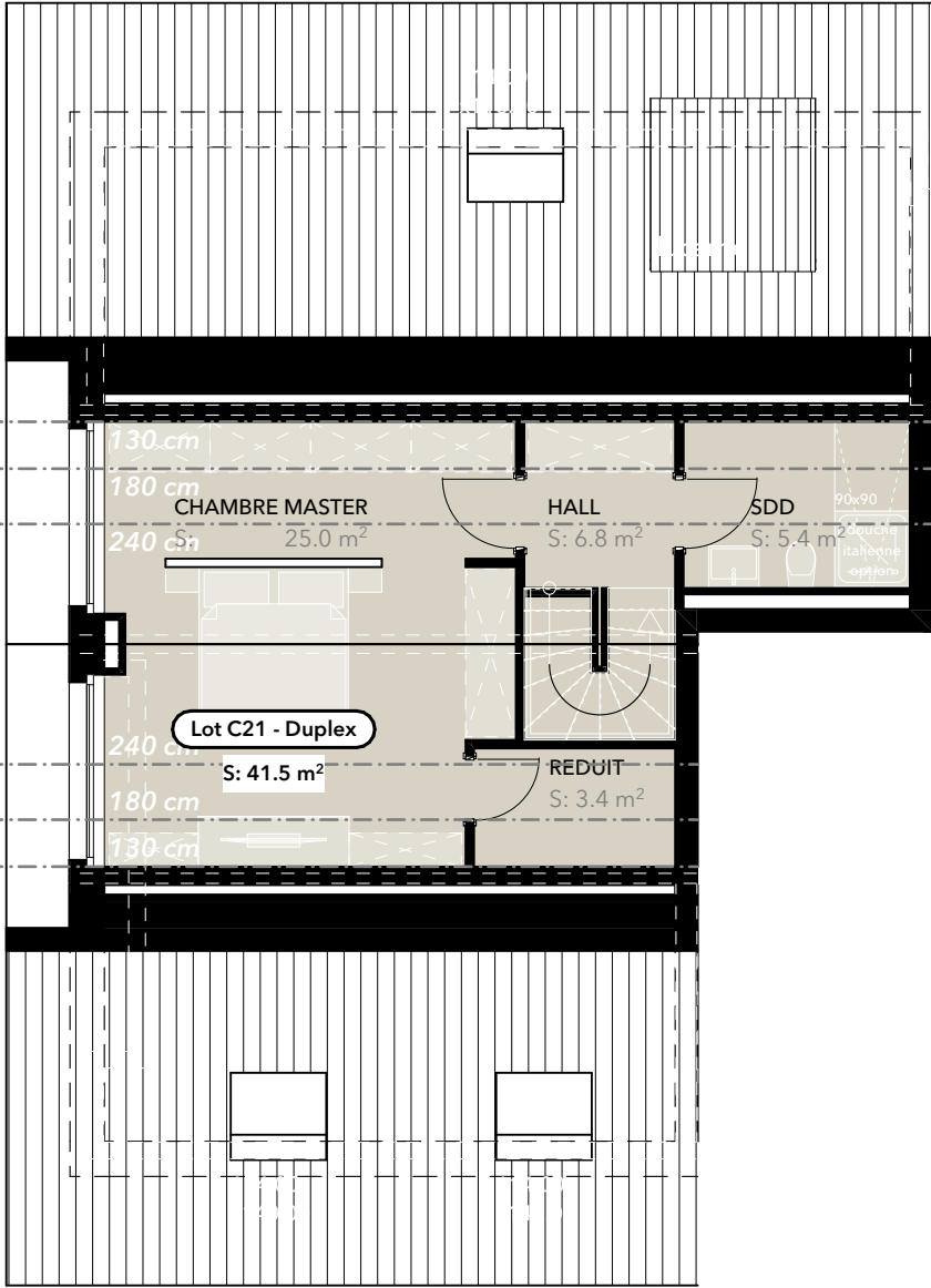
Mezzanine - C21
